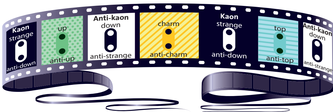
Quantum physics is behind this bizarre transformation act. A kaon can switch between being itself and being its anti-self – from kaon to anti-kaon and back again. All quark families known today must contribute to the process where in a few cases the symmetry will be broken. The explanation of how this happens has given Koboyashi and Maskawa this year's Nobel Prize in Physics.
